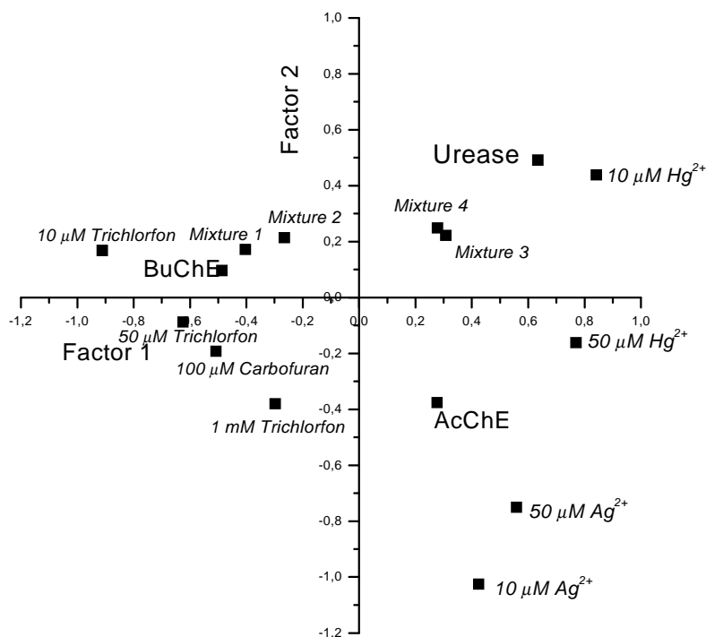
Figure 6. Representation of data from Table 4 by using multivariate correspondence analysis.
