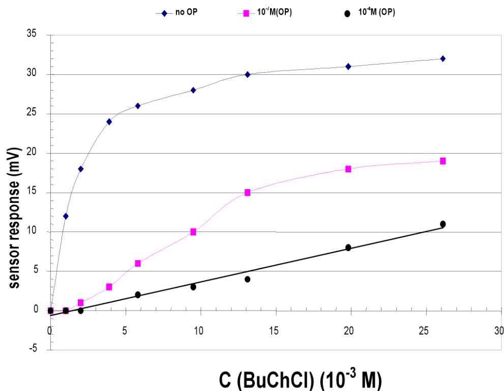
Figure 5. Inhibition effect on the response of the ENFET with a mixed BuChE/ODA LB film by trichlorfon.
