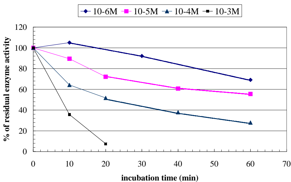
Figure 2. Inhibition effect on the BuChE-BSA FET sensor by trichlorfon. Percent of residual enzyme activity as a function of incubation time.
