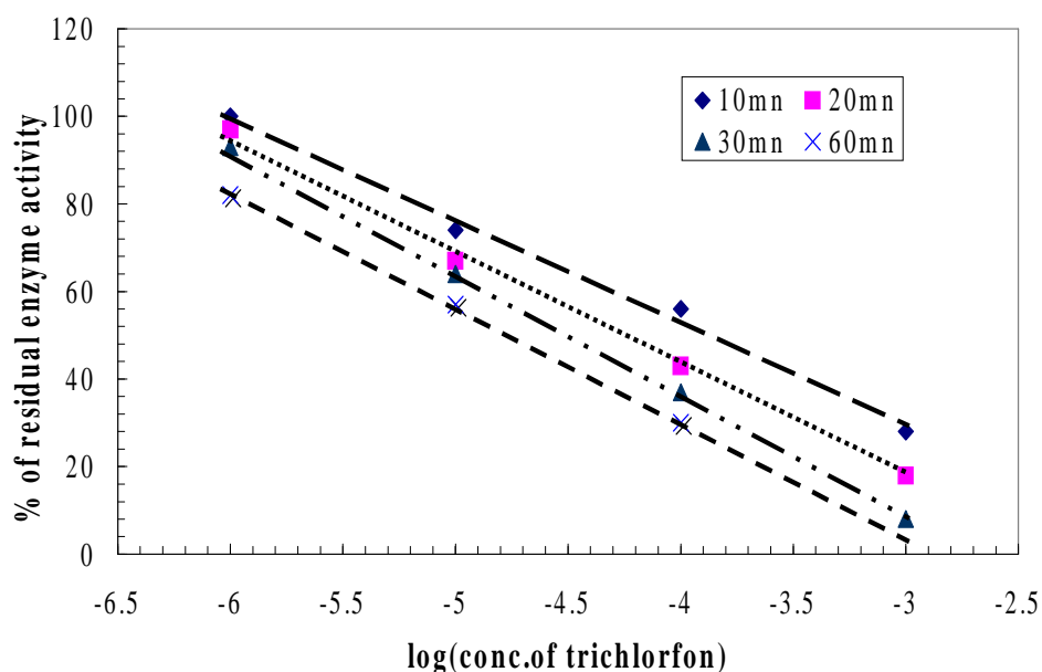
Figure 3. Inhibition effect on the BuChE-BSA FET sensor by trichlorfon. Percent of residual enzyme activity as a function of trichlorfon concentration.
