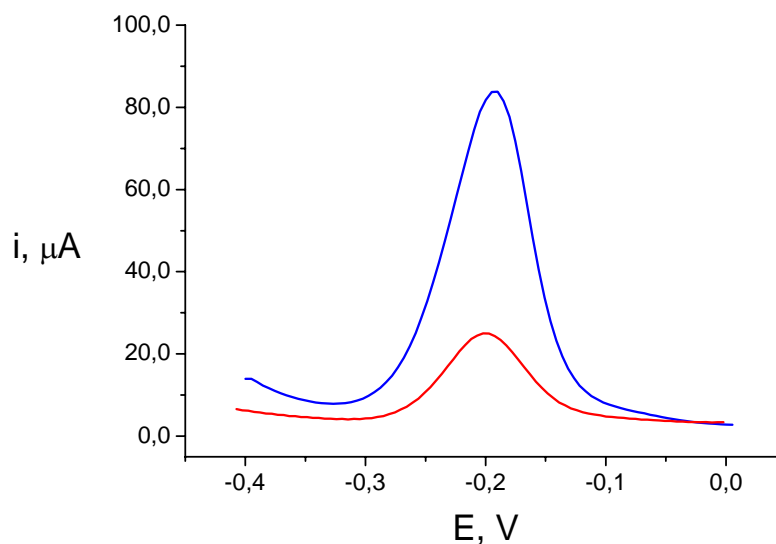
Figure 5. Stripping voltammograms obtained with the ss-DNA-EDC/NHSS-MPA-AuE (—) and with the ds-DNA-EDC/NHSS-MPA-AuE (—) after accumulation of MB. Supporting electrolyte: 50 mM Tris-HCl, 20 mM NaCl (pH 7.2). Immobilization conditions: 2.5 μg DNA, 24 h drying time. Accumulation conditions: [MB] = 75 μM, t_{\text{acc}} = 1 min, open circuit. Measurement conditions: SWV, E_{\text{sw}} = 30 mV, f = 100 Hz, v = 500 mV s -1 .
