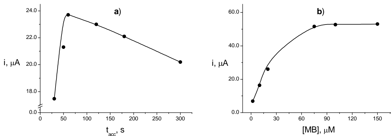
Figure 3. Effect of the accumulation time (a) and MB concentration (b) on the MB anodic stripping SW peak current at the ss-DNA-EDC/NHSS-MPA-AuE. Supporting electrolyte: 50 mM Tris-HCl, 20 mM NaCl (pH 7.2). Accumulation conditions: [\text{MB}] = 20 \mu\text{M} (a), t_{\text{acc}} = 1 \text{ min} (b), open circuit. Measurement conditions: SWV, E_{\text{sw}} = 30 \text{ mV} , f = 100 \text{ Hz} , v = 500 \text{ mV s}^{-1} .
