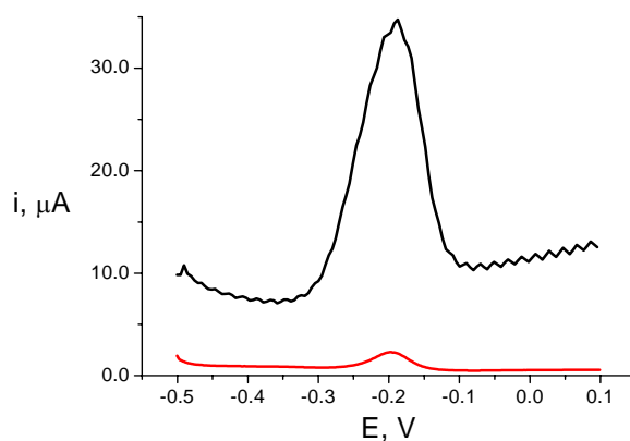
Figure 2. Stripping voltammograms obtained with the ss-DNA-EDC/NHSS-MPA-AuE after accumulation of MB. Supporting electrolyte: 50 mM Tris-HCl, 20 mM NaCl (pH 7.2). Accumulation conditions: [\text{MB}] = 20 \mu\text{M} , t_{\text{acc}} = 5 \text{ min} , open circuit. Measurement conditions: SWV (—), E_{\text{sw}} = 30 \text{ mV} , f = 100 \text{ Hz} , v = 500 \text{ mV s}^{-1} , and DPV (—) 20 \text{ mV s}^{-1} , \Delta E = 20 \text{ mV} .
