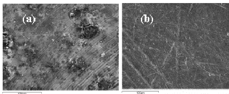
Figure 6. Scanning electron micrographs obtained for an ss-DNA-EDC/NHSS-MPA-AuE before (a) and after (b) accumulation of MB. Immobilization conditions: 2.5 µg DNA, 24 h drying time. Accumulation conditions (b): [MB] = 75 µM, t_{acc} = 1 min, open circuit.
