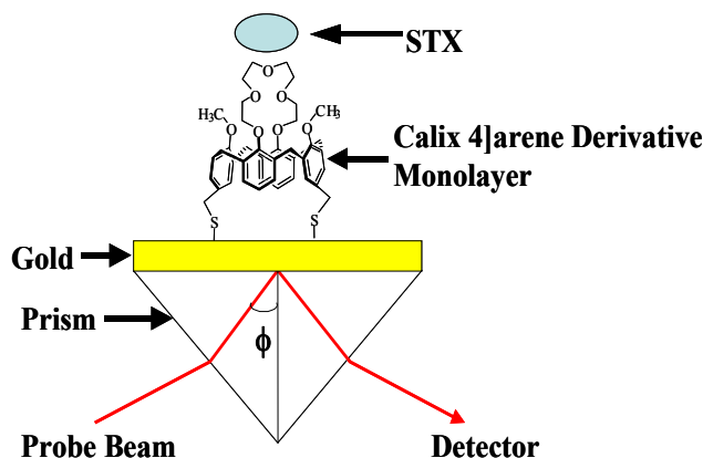
Figure 3. Schematic diagram of the sensor chip configuration.
