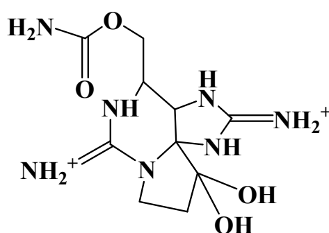
Figure 1. Molecular structure of saxitoxin.
