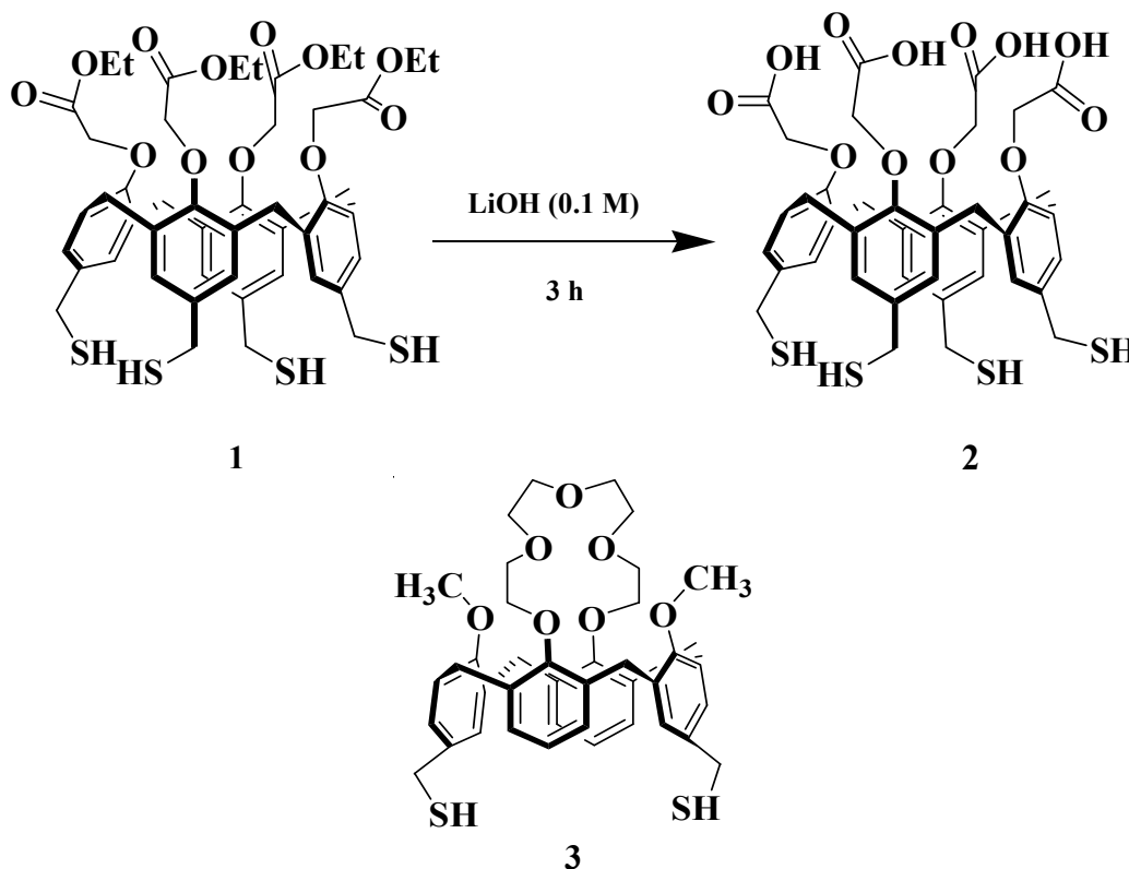
Figure 2. Molecular structure of calix[4]arene derivatives used in this study.
