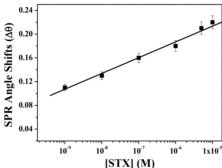
Figure 5. Relative SPR angle shifts of 3 SAM corresponding to various concentration of STX. Linear regression shows a working range of 1.0 \times 10^{-9} - 1.0 \times 10^{-5} M ( r^2 = 0.994 ).
