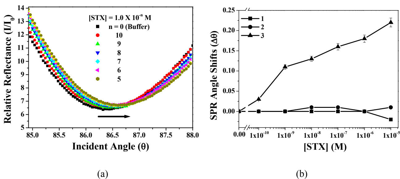
Figure 4. (a) SPR spectra of 3 SAM in the presence of various concentrations of STX; (b) relative SPR angle shifts of calix[4]arene derivatives corresponding to the presence of various concentration of STX.
